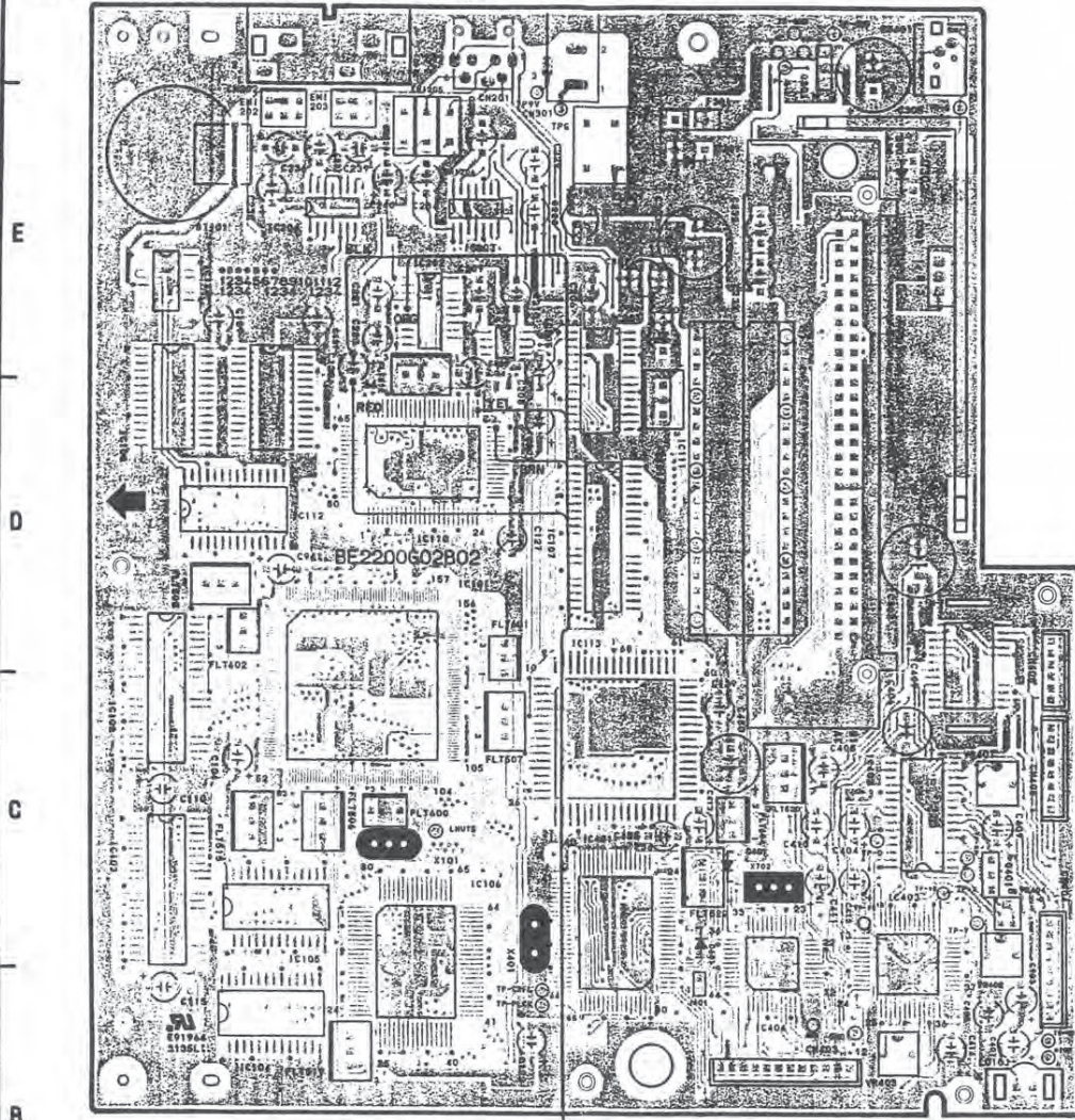
11-1. Main Circuit Board(Top View)
